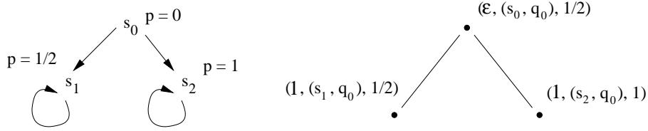
Fig. 2. Example Kripke structure M and accepting run
