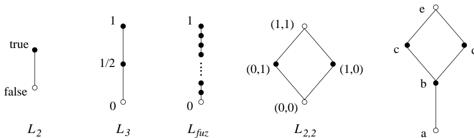
Fig. 1. Some distributive lattices
